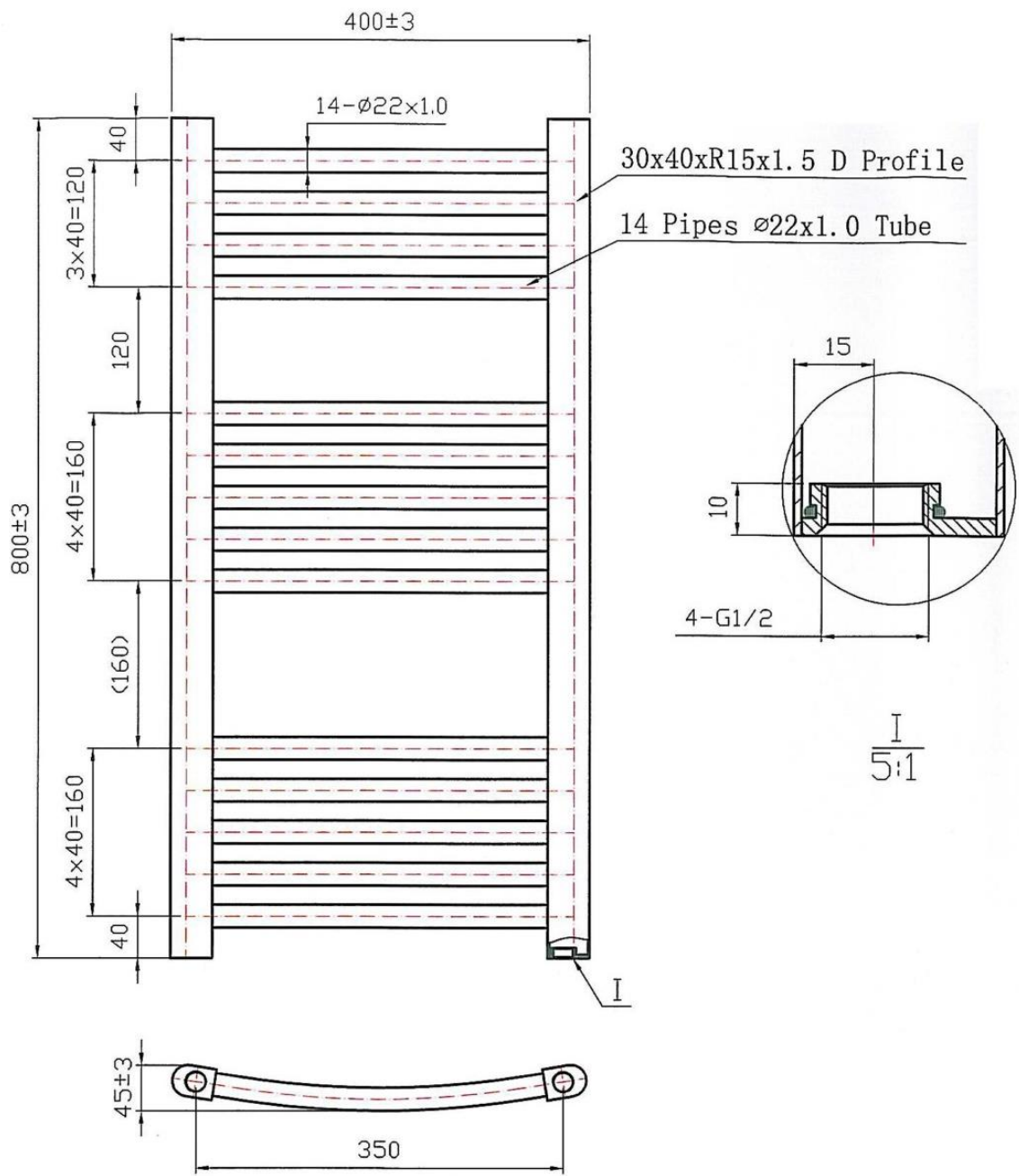
800*400 14 pipes Curved
